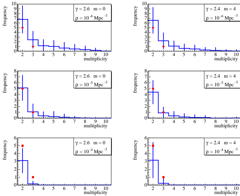
Figure 3. Small scale anisotropies simulated in 13 for the AGASA statistics. The thick dots represent the number of doublets and triplets actually observed.
